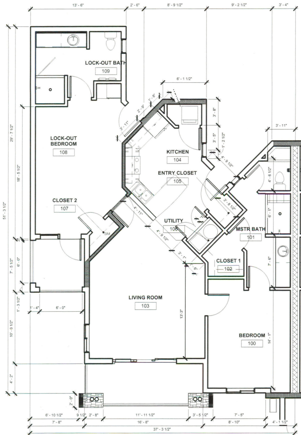
CASAS AT MIRA VISTA FLOOR PLAN 1200 SF 1/8" = 1'-0"
